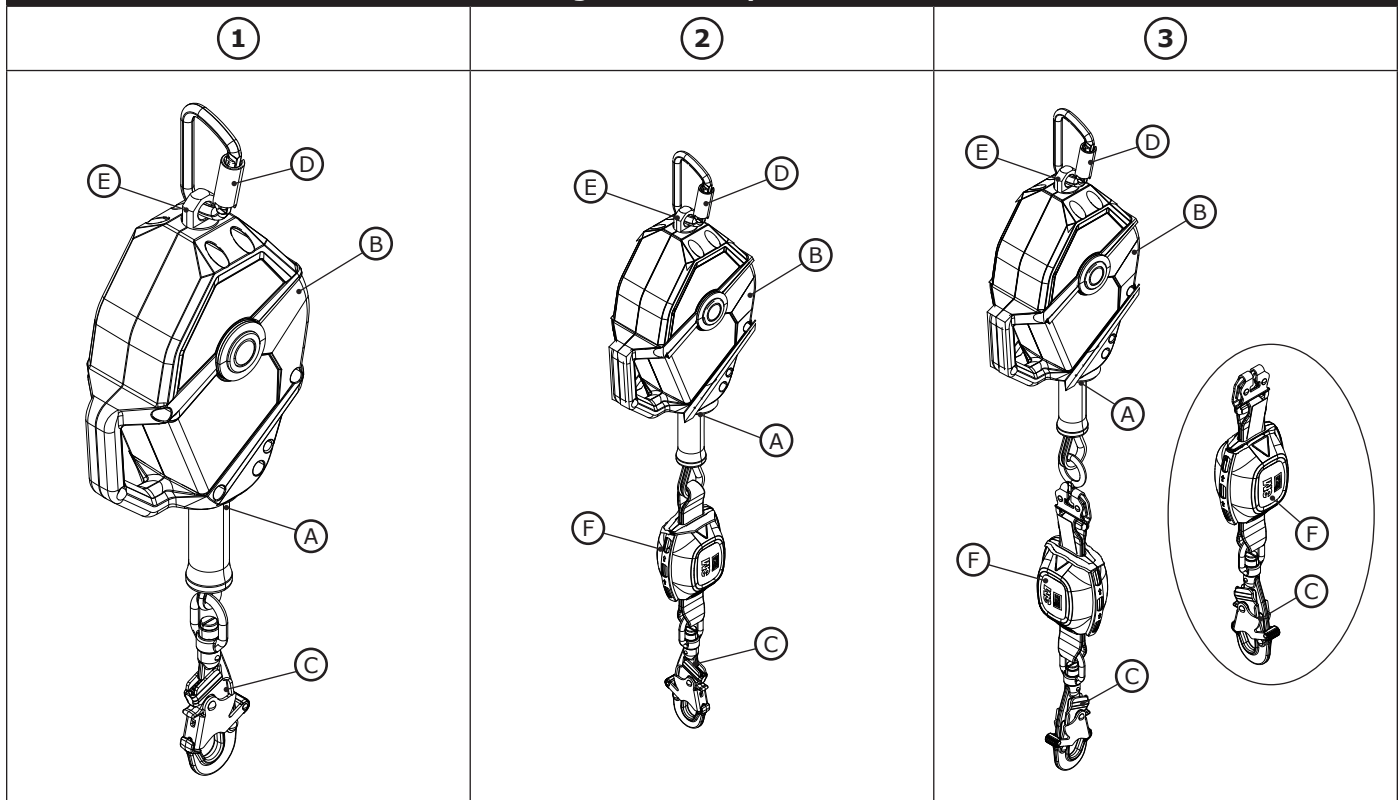
Figure 2 - Components
