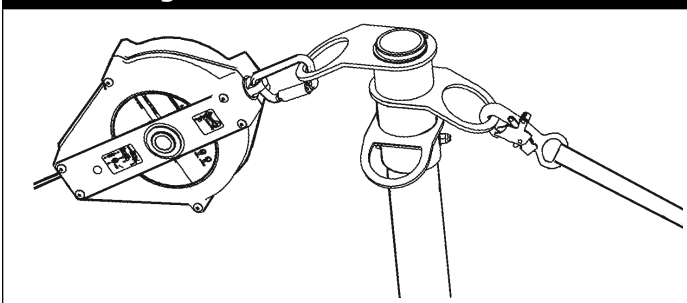
Figure 7 - Connection to Anchor
