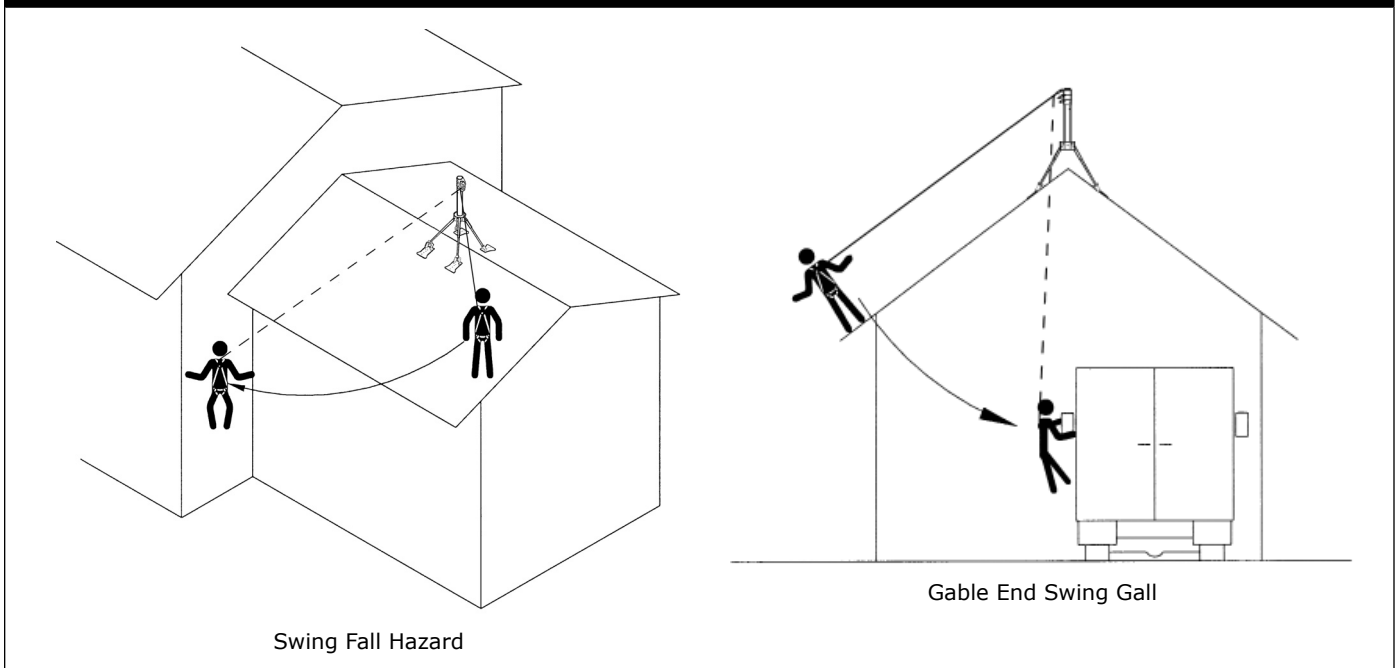
Figure 4 - Swing falls
