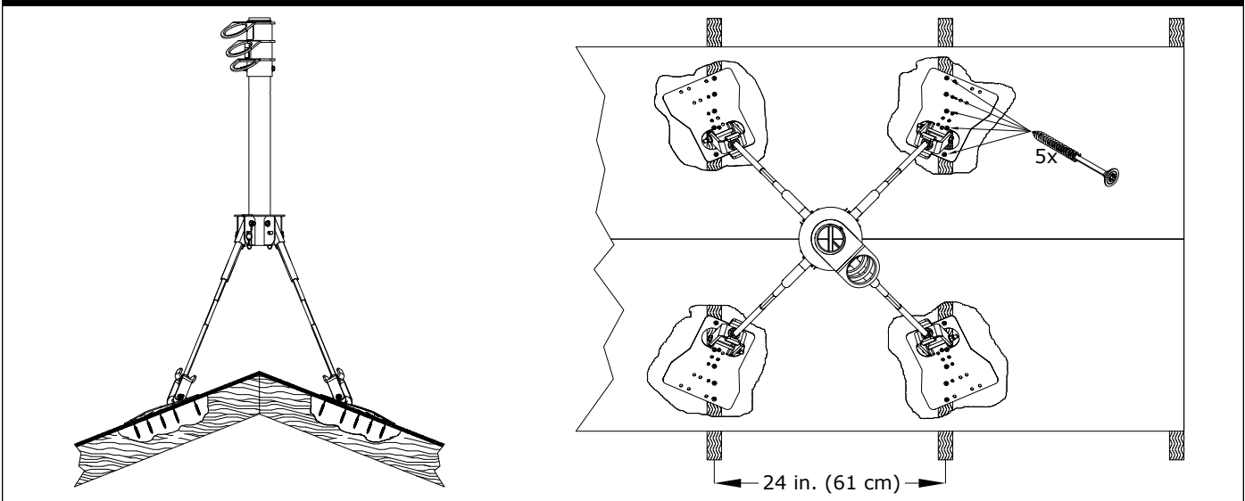
Figure 6 - Attaching the Roof Anchor
