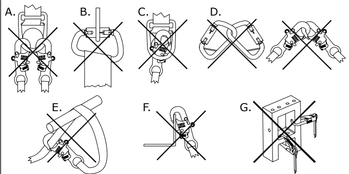
Figure 3 - Inappropriate Connections
